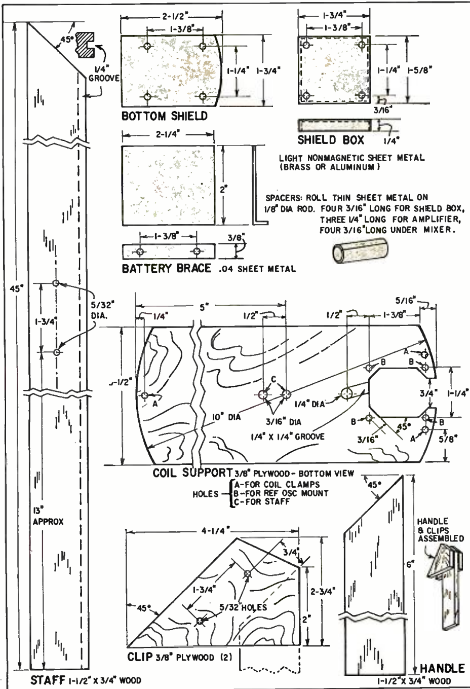
Fig. 3—The sheet-metal parts, pattern for the coil support, and the remaining wood parts.
