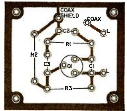
Fig. 2—Layout of boards author made. Perforated phenolic board can be used equally well, or even point-to-point wiring. Boards are viewed from top with printed circuit (underside) in gray. To make patterns for your boards, trace on tissue paper and then reverse and use as templates.
